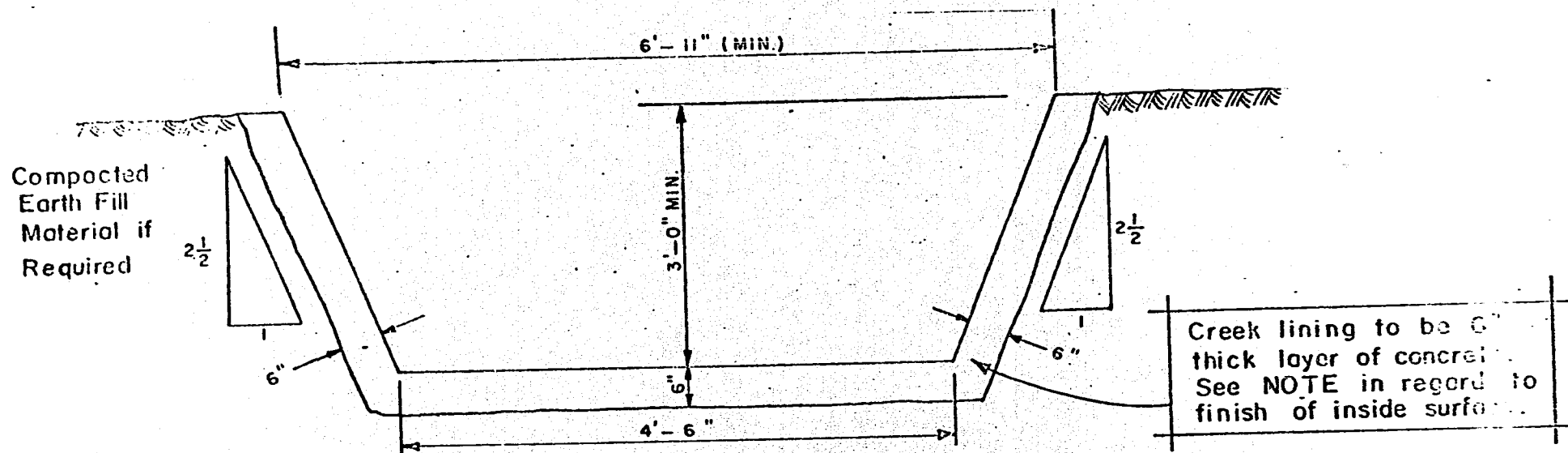
TYPICAL CREEK CROSS-SECTION
